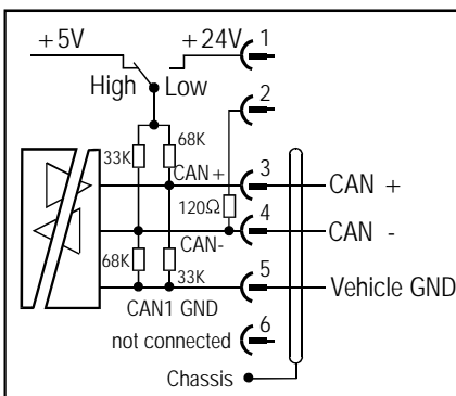
CAN-Anschluß High Speed CAN-connection High Speed
